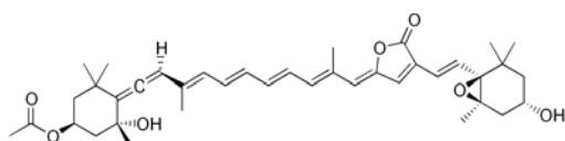
Peridinina (carotenoide)
